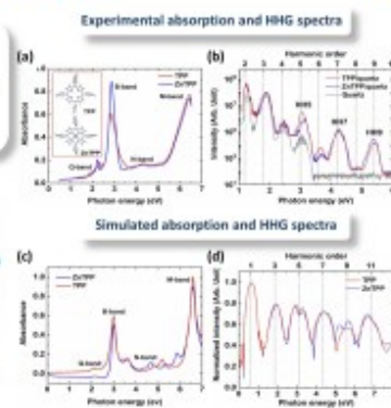
Snapshots of the time-dependent differential electron density of TPP and ZnTPP. 5
