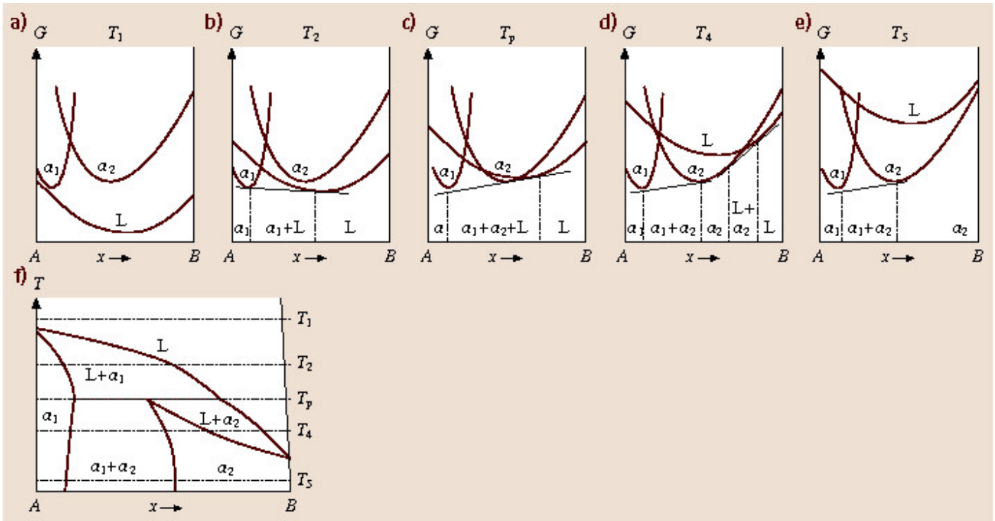
Peritectic phase diagram and Gibbs free energy curves
