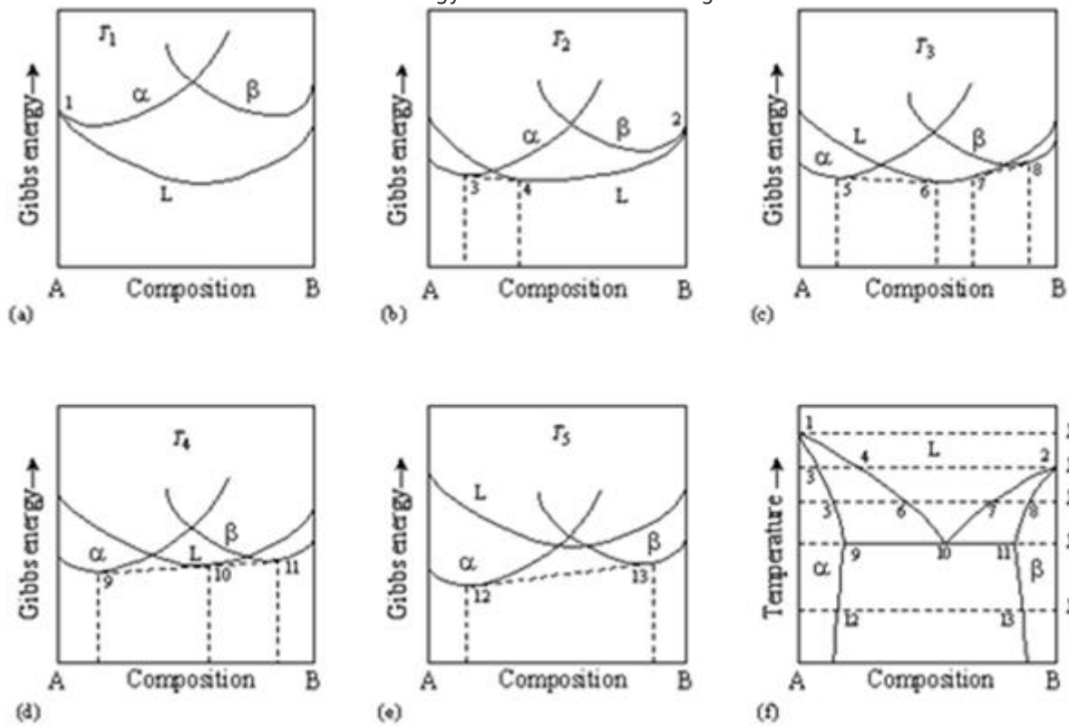
Eutectic Phase diagram and Gibbs free energy curves
