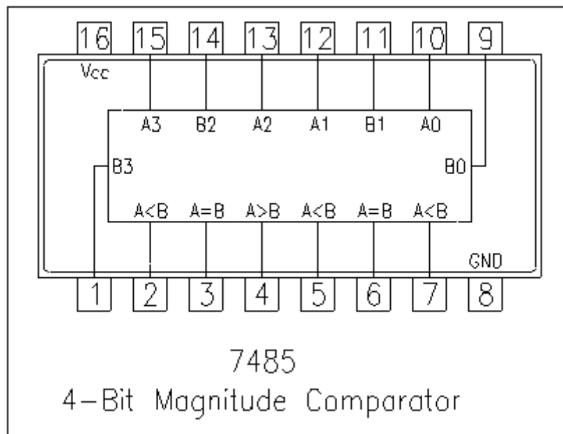
4-bit magnitude comparator - iC 74HC85
