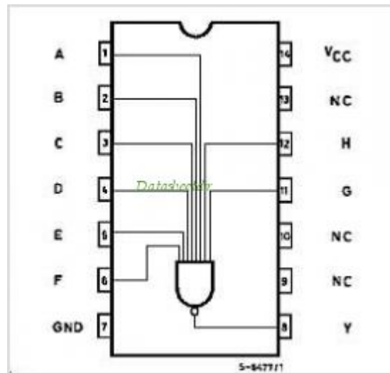
IC 74HC30 - 8-input NAND gate
