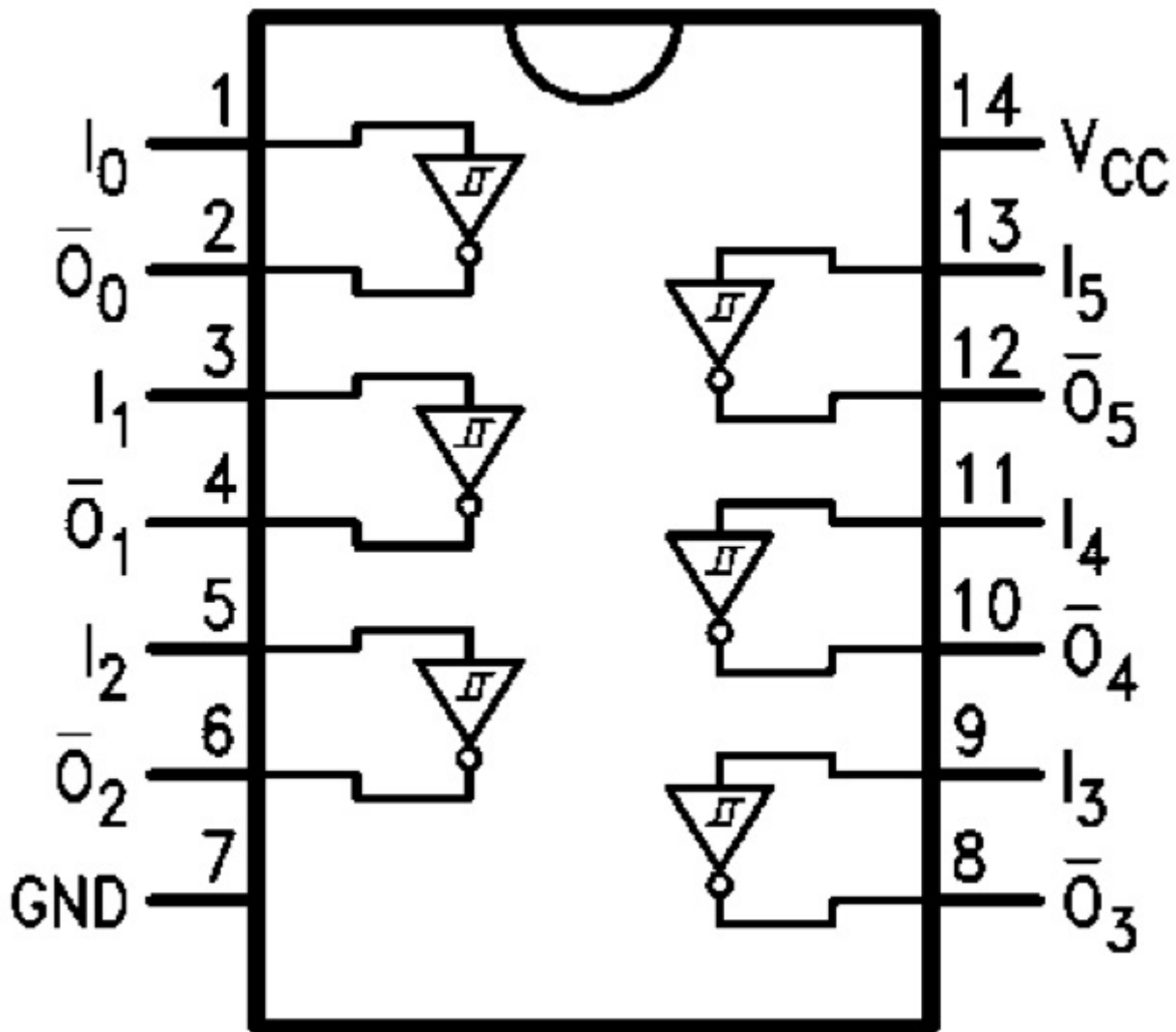
74HC14 -Hex inverting Schmitt trigger
