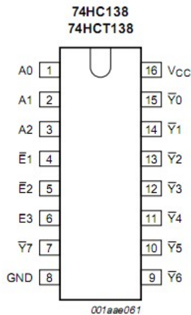
74HC138 3-to 8- line decoder pin diagram
